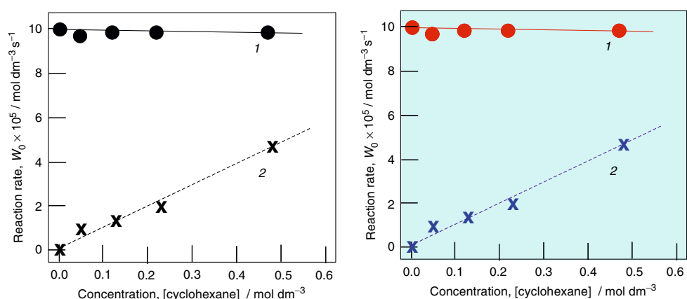
Fig. 9 Competitive oxidation of dec-1-ene ( 0.25 \text{ mol dm}^{-3} ) and cyclohexane. Initial rates of the formation of dec-1-ene epoxide (curve 1) and a sum of cyclohexanone and cyclohexanol (curve 2) versus concentration of cyclohexane in the oxidation by PAA ( 0.72 \text{ mol dm}^{-3} ) in MeCN at 25^\circ\text{C} catalyzed with 1 ( 5 \times 10^{-5} \text{ mol dm}^{-3} )
